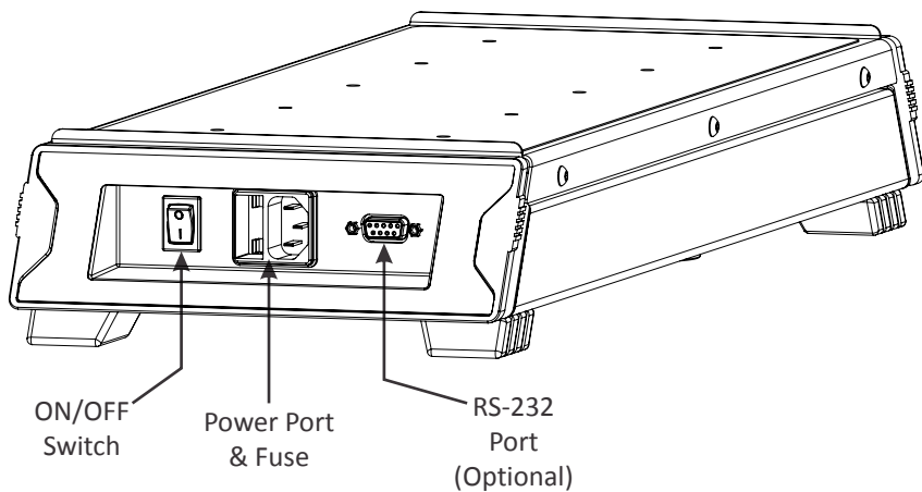
Rear Side
